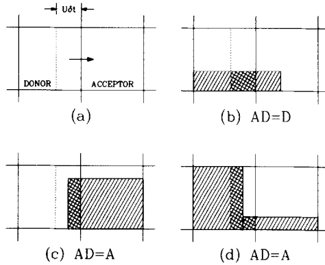
FIG. 5. Examples of free surface shapes used in the advection of F . The donor–acceptor arrangement is shown in (a), where the dashed line indicates the left boundary of the total volume being advected. The cross-hatched regions shown in (b–d) are the actual amounts of F fluxed.
