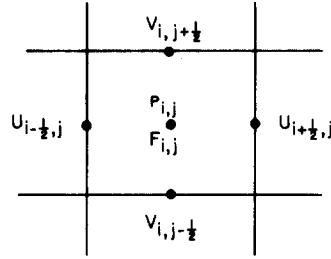
FIG. 2. Location of variables in a typical mesh cell.
