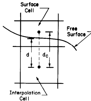
FIG. 4. Sketch showing definition of quantities used in defining free surface pressure boundary condition.
