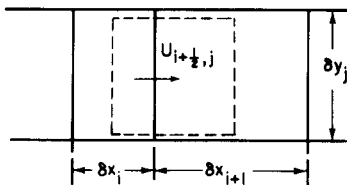
FIG. 3. Control volume (dashed rectangle) used for constructing a finite-difference approximation for the u momentum equation at location (i + 1/2, j) .
