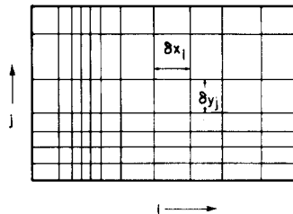
FIG. 1. Schematic of finite-difference mesh with variable rectangular cells.
