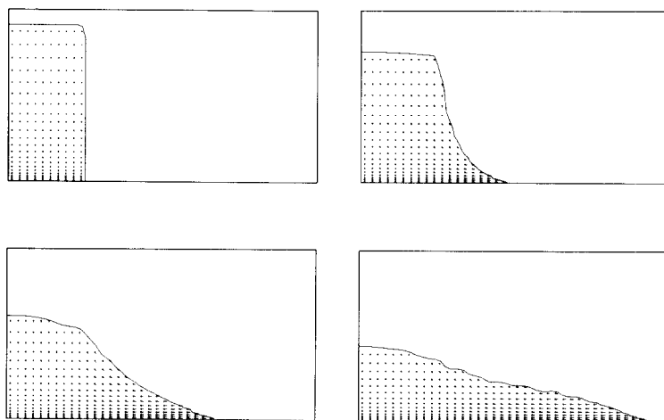
FIG. 6. Velocity vectors and fluid configurations for broken dam problem at times 0.0, 0.9, 1.4, and 2.0. Vectors are drawn from cell centers, which are marked by + signs. The free surface is drawn as an F = \frac{1}{2} contour line, which is why the top right corner at t = 0.0 is not 90^\circ .
