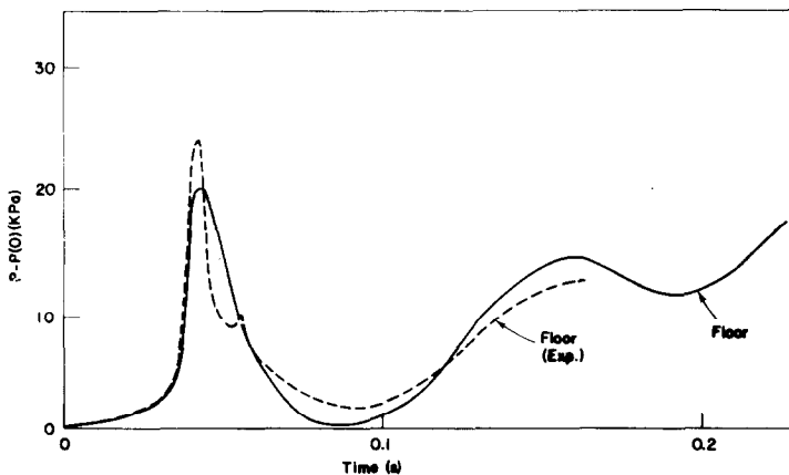
FIG. 14. Comparison of calculated and measured pressure history on floor of pool chamber.
