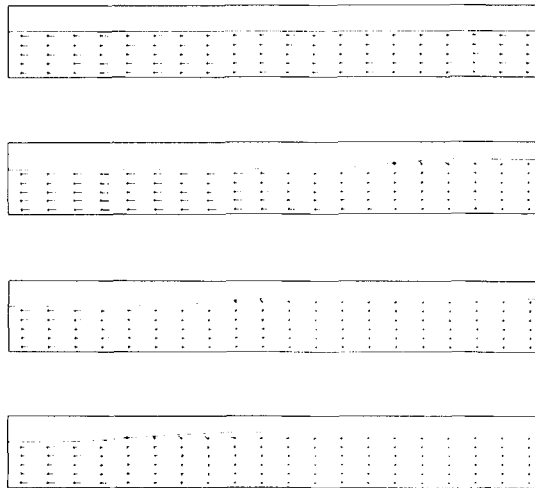
FIG. 8. Velocity vectors and fluid configuration for undular bore problem at times 0.0, 4.05, 7.02, and 10.08.
