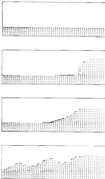
FIG. 9. Velocity vectors and fluid configuration for breaking bore problem at times 0.0, 6.50, 8.51, and 14.01.
