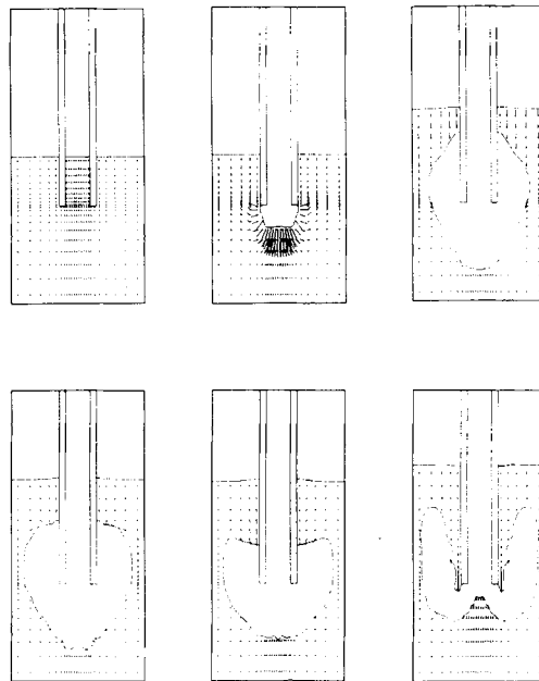
FIG. 13. Velocity vectors and free surface configurations computed when air is forced through submerged vent pipe.
