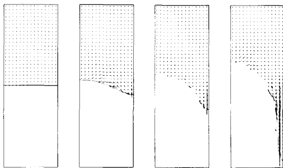
FIG. 10. Evolution of a Rayleigh-Taylor instability started by a pressure perturbation. Times are 0.0, 0.4, 0.8, and 1.6.
