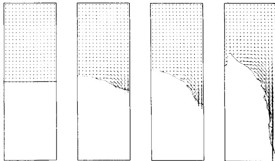
FIG. 11. Repeat of calculation shown in Fig. 10 using pure acceptor cell advection for F . Note the considerably more irregular surface in the last frame.
