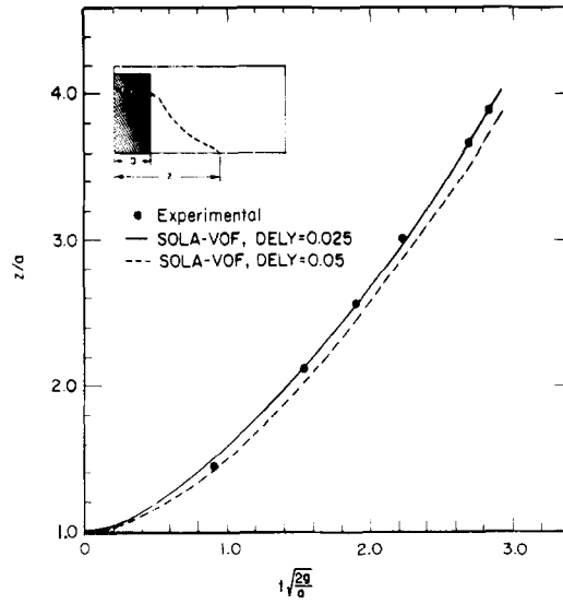
FIG. 7. Comparison of calculated results with experimental data for the broken dam problem.
